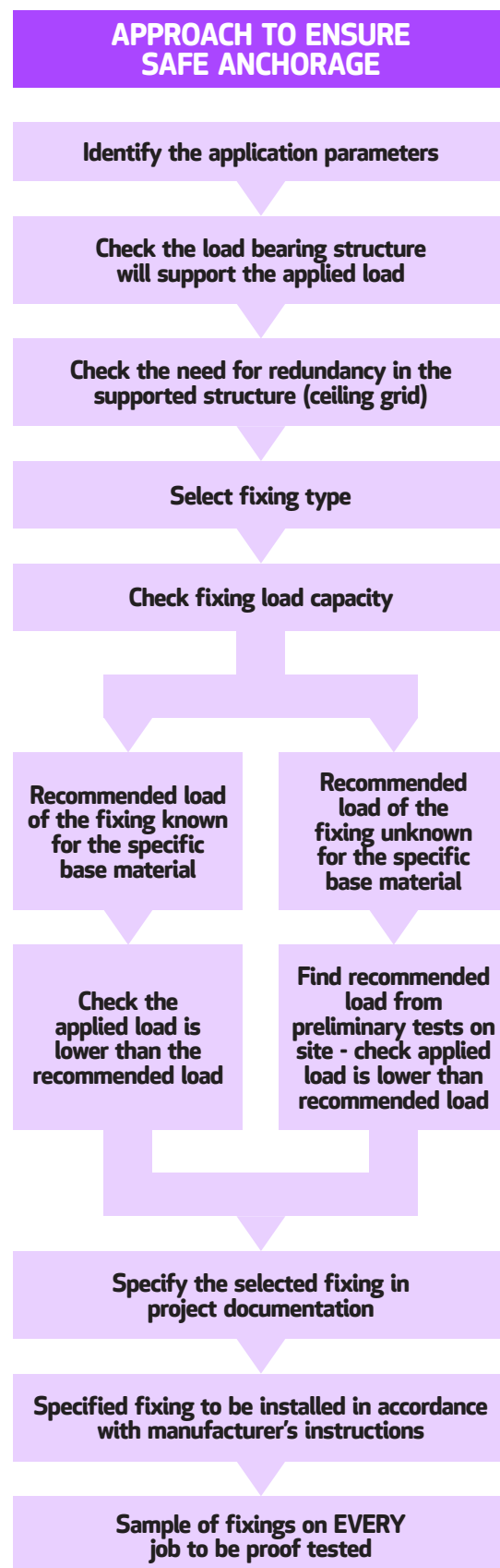
Figure 30 Approach to ensure safe anchorage (from the FIS and CFA Best Practice Guide 'Selection and installation of top fixings for suspended ceilings'.
